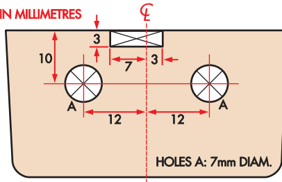
RIGHT-HAND END (OUTSIDE VIEW)
