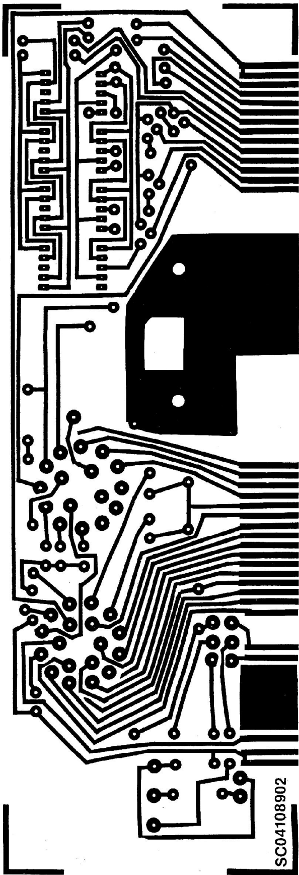
Figs.7-10: here are actual size artworks for the two PC boards, the front panel and the light mask.
