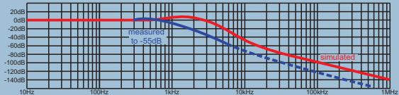
V out versus Frequency
