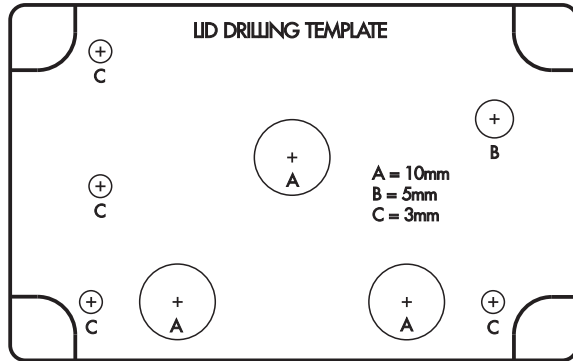
Unmarked holes 3mm diameter (4 places), 5mm (1 place)
