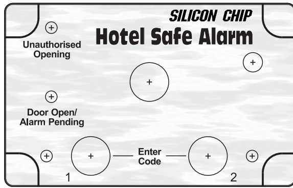
Unmarked holes 3mm diameter (4 places), 5mm (1 place)
