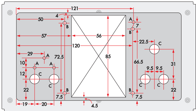
HOLES A: 3.0mm DIAMETER; HOLES B: 3.5mm DIAMETER; HOLES C: 10mm DIAMETER
