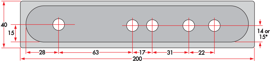
REAR PANEL DRILLING DETAILS (SHOWN HERE AT 50% OF FULL SIZE) ALL HOLES ARE 10mm DIAMETER
