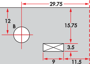
REAR OF HB-5062 BOX
