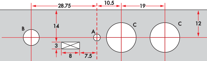
FRONT OF JAYCAR HB-5062 BOX (111 x 60 x 30)
