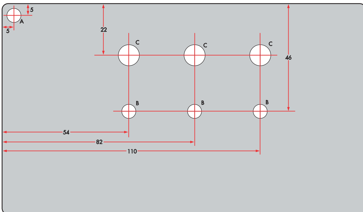
TOP OF CASE DRILLING
