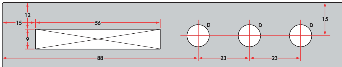
CASE FRONT PANEL CUTTING & DRILLING
