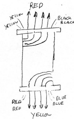
FORMER 2 UNDERSIDE VIEW
