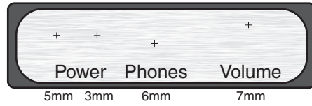
End Panel Drill Guide
